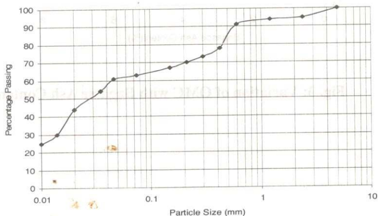
Fig. 1: Particle size distribution curve for the natural soil
