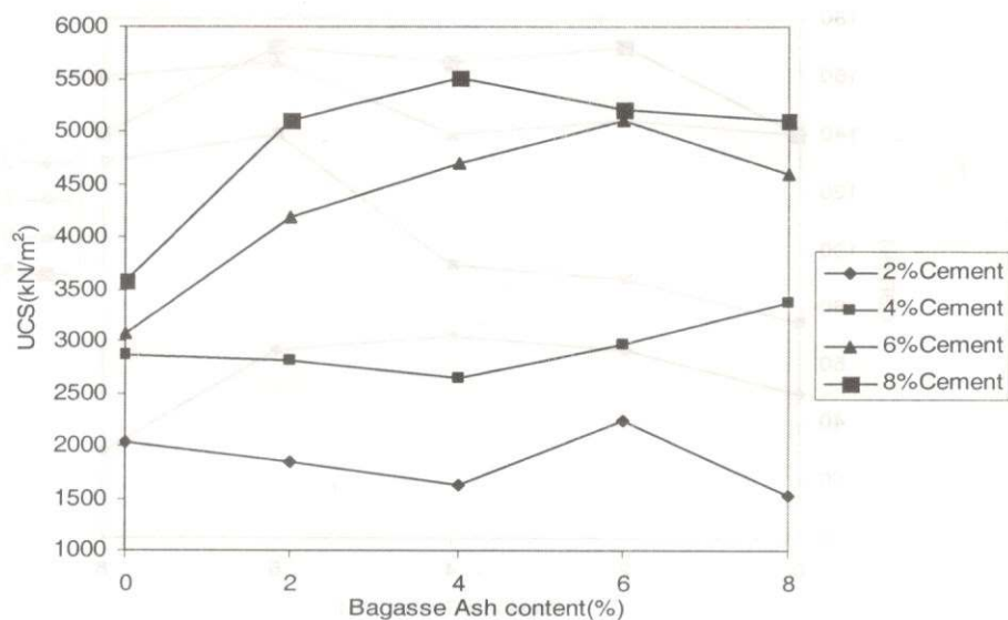
Fig. 6: Variation of UCS with Bagasse Ash Content for 14 days Curing Period
