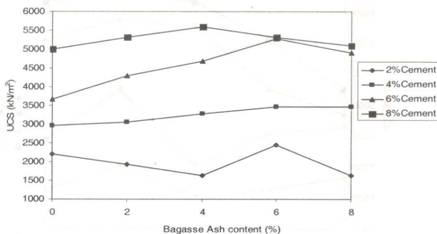
Fig. 7: Variation of UCS with Bagasse Ash Content for 28 days Curing Period
