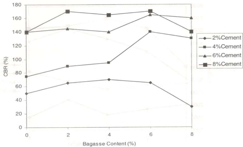
Fig. 4: Variation of CBR with Bagasse Ash Content
