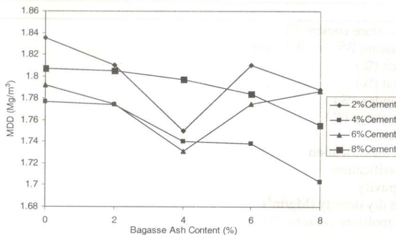
Fig. 2: Variation of MDD with Bagasse Ash Content
