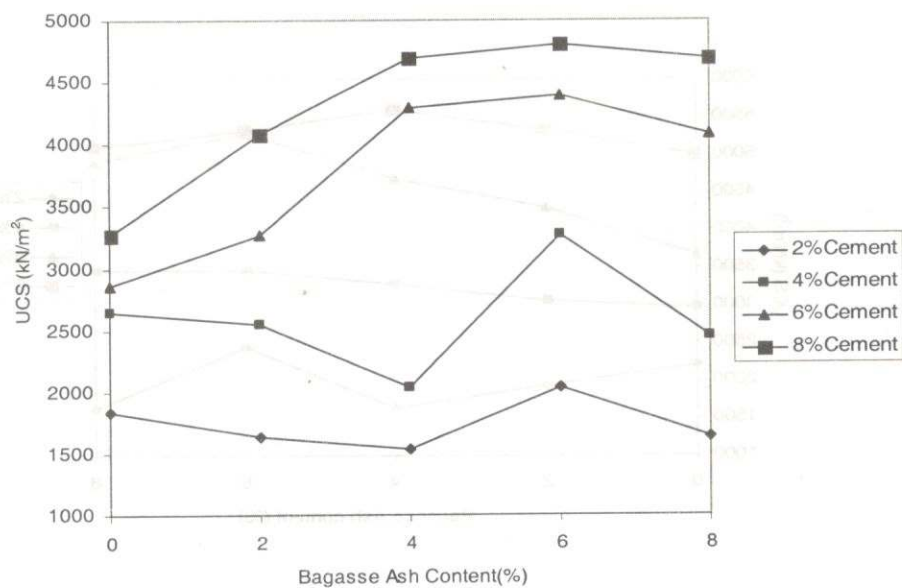
Fig. 5: Variation of UCS with Bagasse Ash Content for 7 days Curing Period
