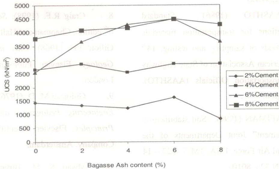
Fig. 8: Variation of UCS for 7 days cured and 7 days soaked with Bagasse Ash Content.
