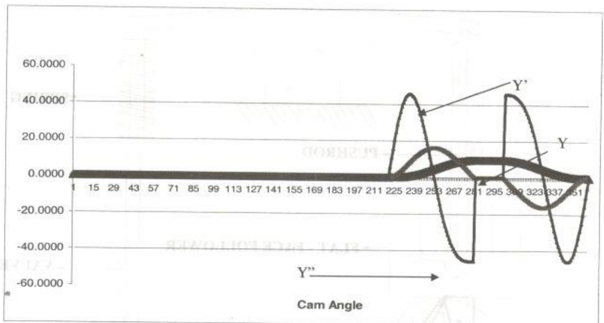
Figure 2: Motion profiles for sample design
