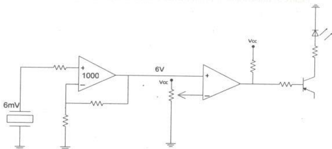
Figure 4b: The Remote Control Circuit
