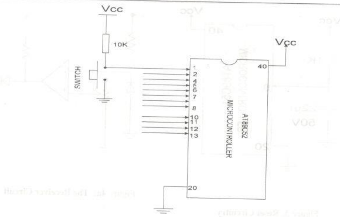
Figure 5: Illustration of Input Switch Connection to the Microcontroller
