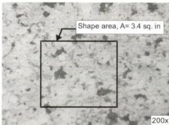
(c) 25% drawn deformation Number grains within area = 60 grains/sq. in ASTM grain size no. = 6.90
