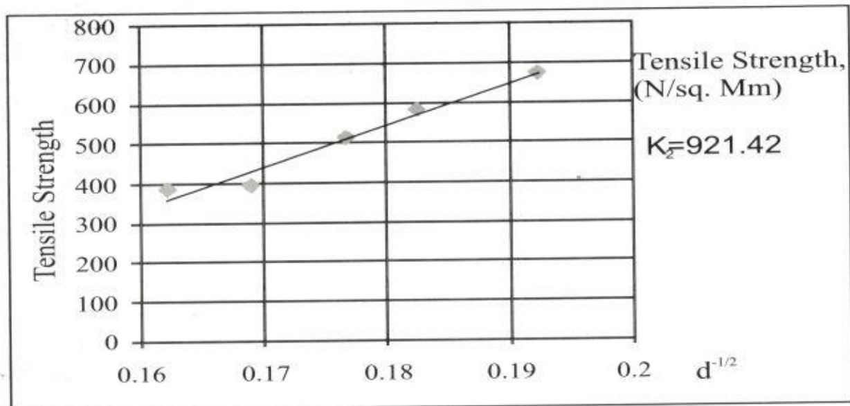
Figure 3. Hall-Petch plot of Tensile strength for cold drawn low carbon steel
