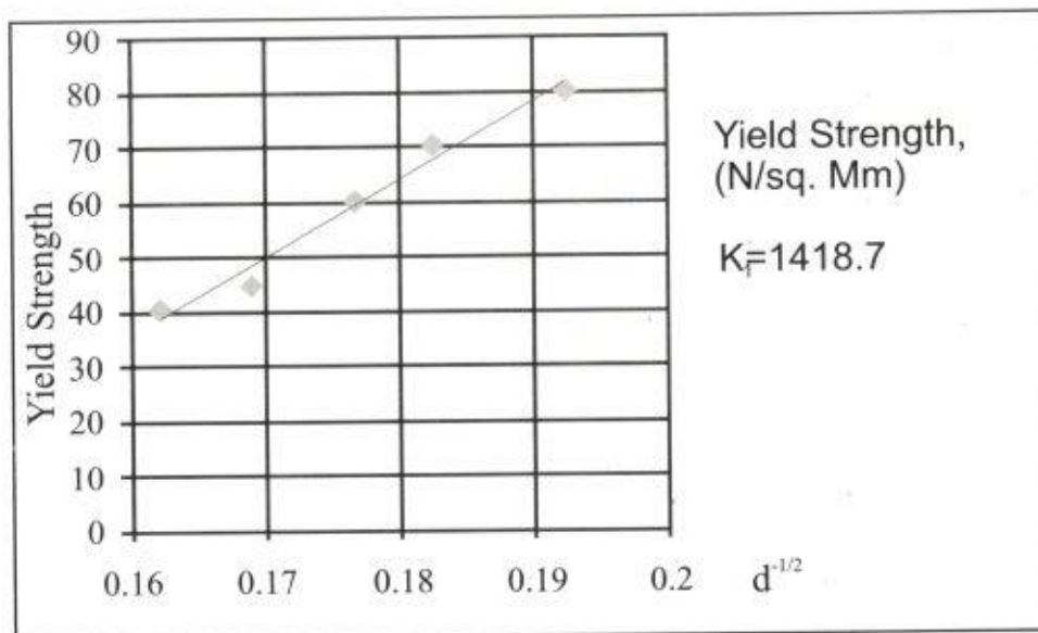
Figure 2. Hall-Petch plot of yield strength for cold drawn low carbon steel
