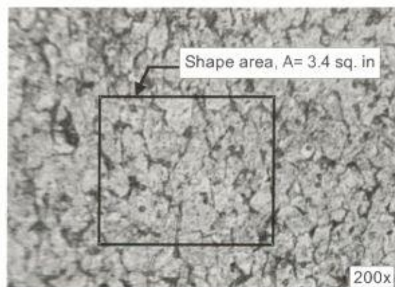
(b) 20% drawn deformation Number grains within area = 71.18 grains/sq. in ASTM grain size no. = 7.15
