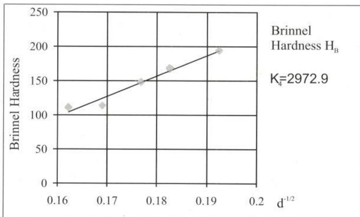
Figure 5. Hall-Petch plot of Brinell Hardness for cold drawn low carbon steel
