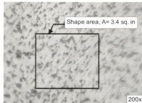
(d) 40% drawn deformation Number grains within area = 51.18 grains/sq. in ASTM grain size no. = 6.67
