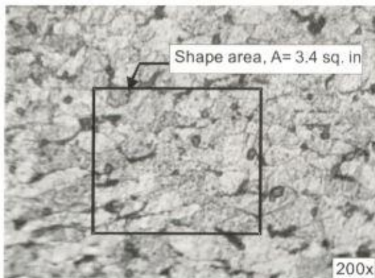
(a) Control specimen Number grains within area = 88.7 grains/sq in ASTM grain size no. = 7.47
