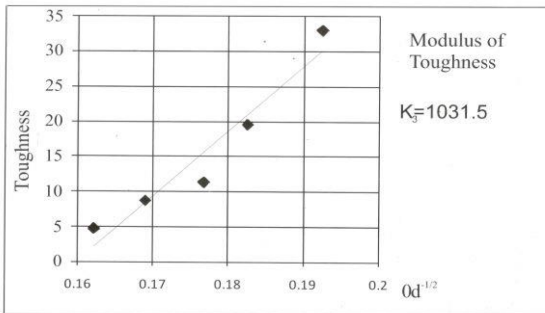
Figure 4. Hall-Petch plot of Toughness for cold drawn low carbon steel
