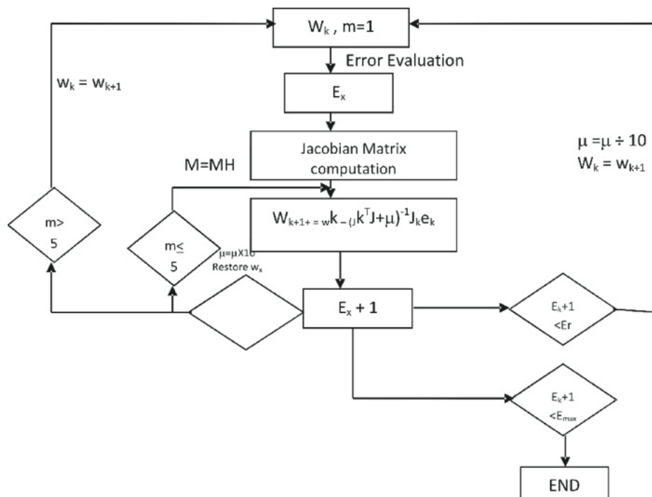
Figure 4.0: Flow Chart for the training process using Levenber – Marquardt algorithm
