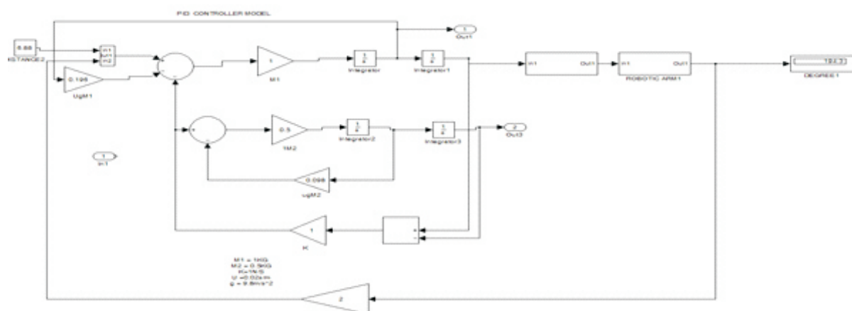
figure 13.0: PID Controller Model
