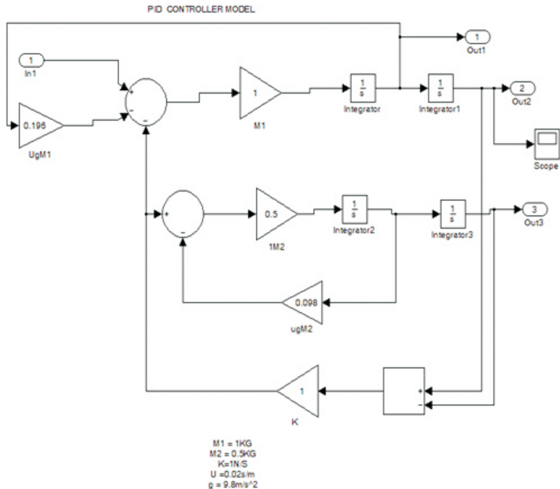
Figure 10.0: Designed Proportional Integral Derivative (PID) model
