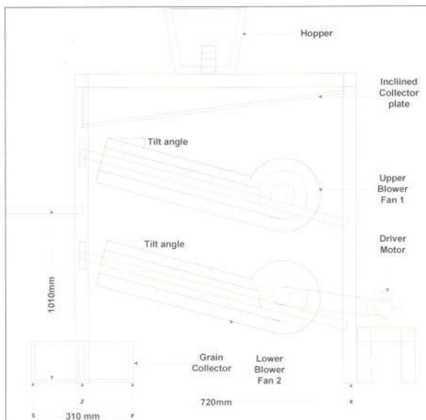
Figure 2: Set up of blower fans at tilt angles during testing
