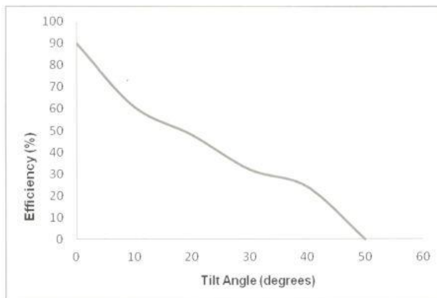
Figure 5: Effeciencies at various tilt angles for fan blower 2
