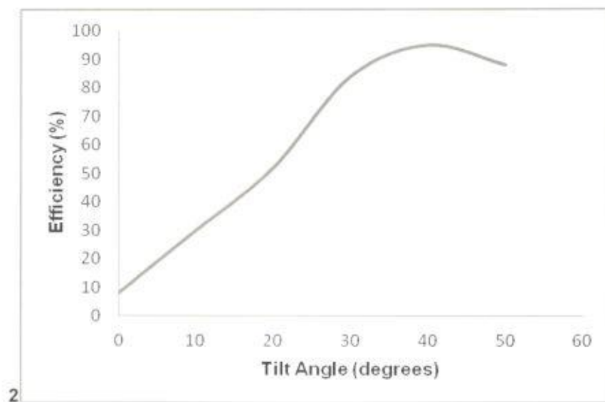
Figure 4: Effeciencies at various tilt angles for fan blower 1
