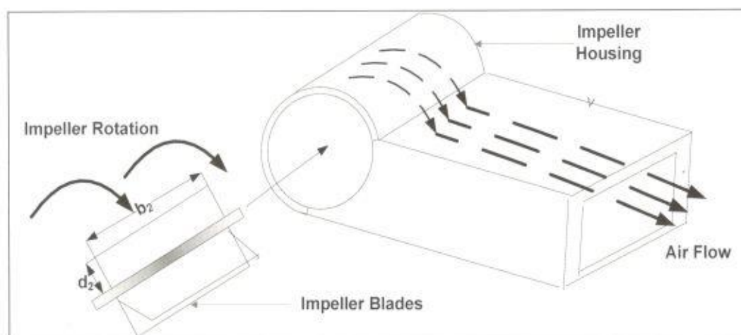
Figure 3: Impeller blade design parameters and its positioning
