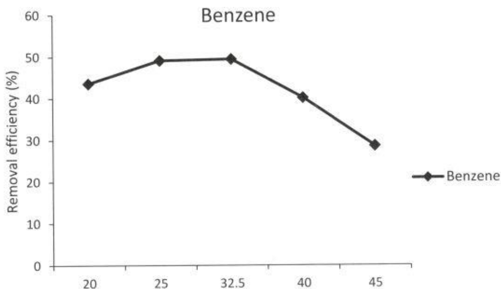
Figure 3: A plot of temperature vs removal efficiency.
