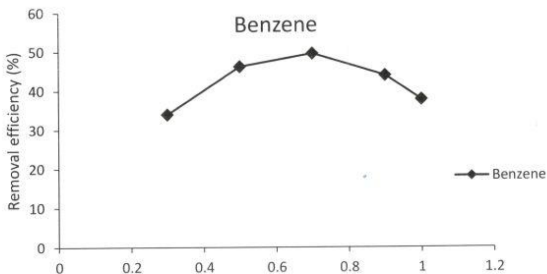
Figure 2: A plot of adsorbent dosage vs removal efficiency.
