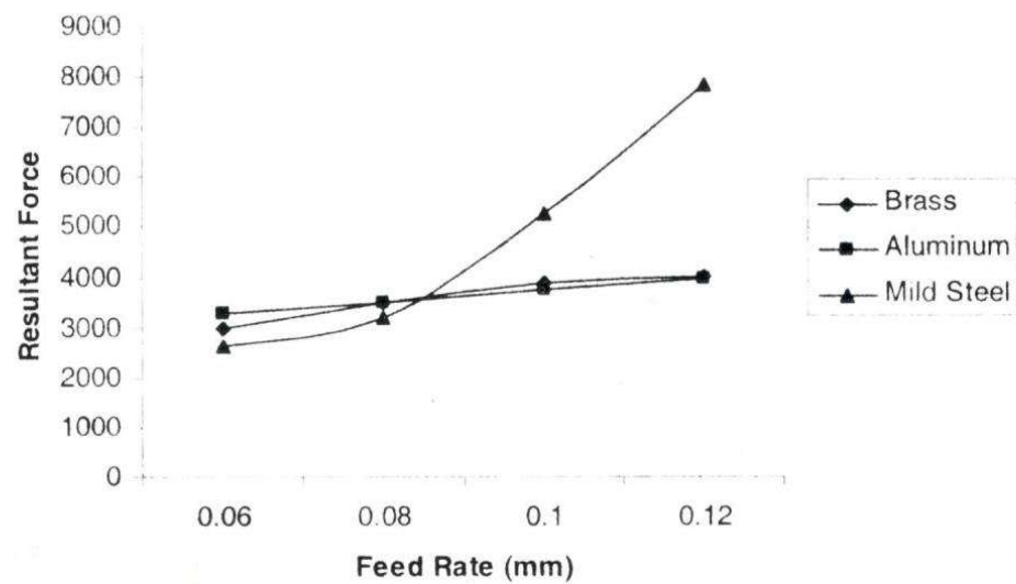
Figure 2: Effects of Feed Rate on Resultant Force at Constant Speed of 4.32m/s
