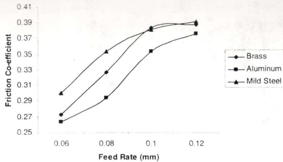
Fig. 1: Effects of Feed Rate on Friction Co-efficient at Constant Speed of 4.32m/s
