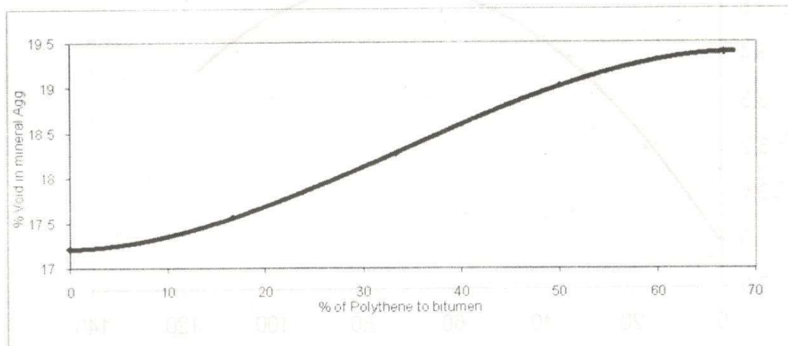
Fig. 3: Variation of Void in mineral Aggregate with % pure water sachet to bitumen
