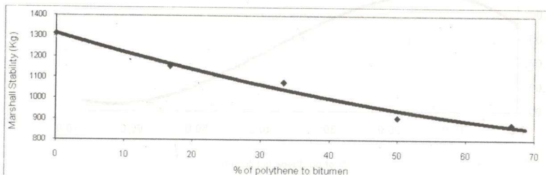
Fig. 6: Variation of Marshall Stability with % pure water sachet to bitumen
