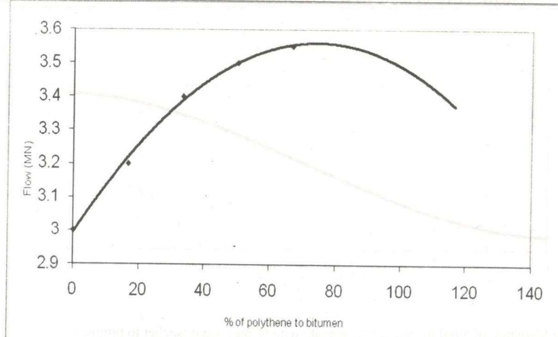
Fig. 5: Variation of Flow with % pure water sachet to bitumen
