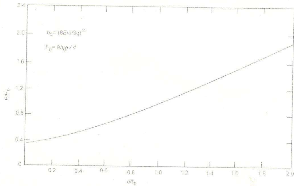
Fig. 4 Single sling case - sling force
