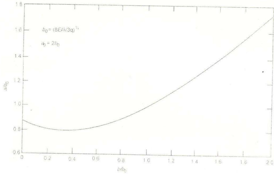
Fig. 3 Single sling case - lifted length
