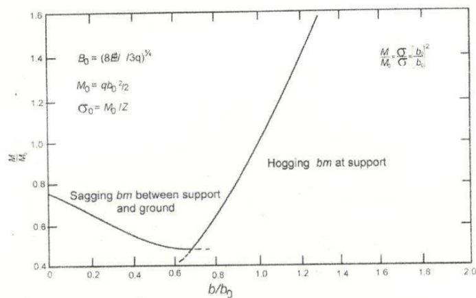
Fig. 5. Single sling case - maximum moment and stress.
