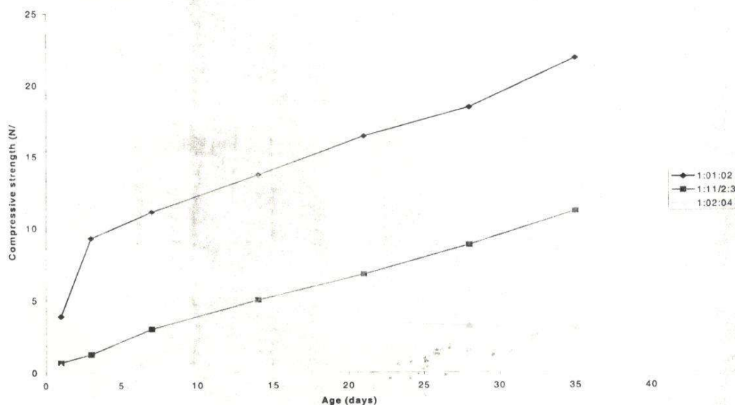
Figure 2: Compressive strength against age
