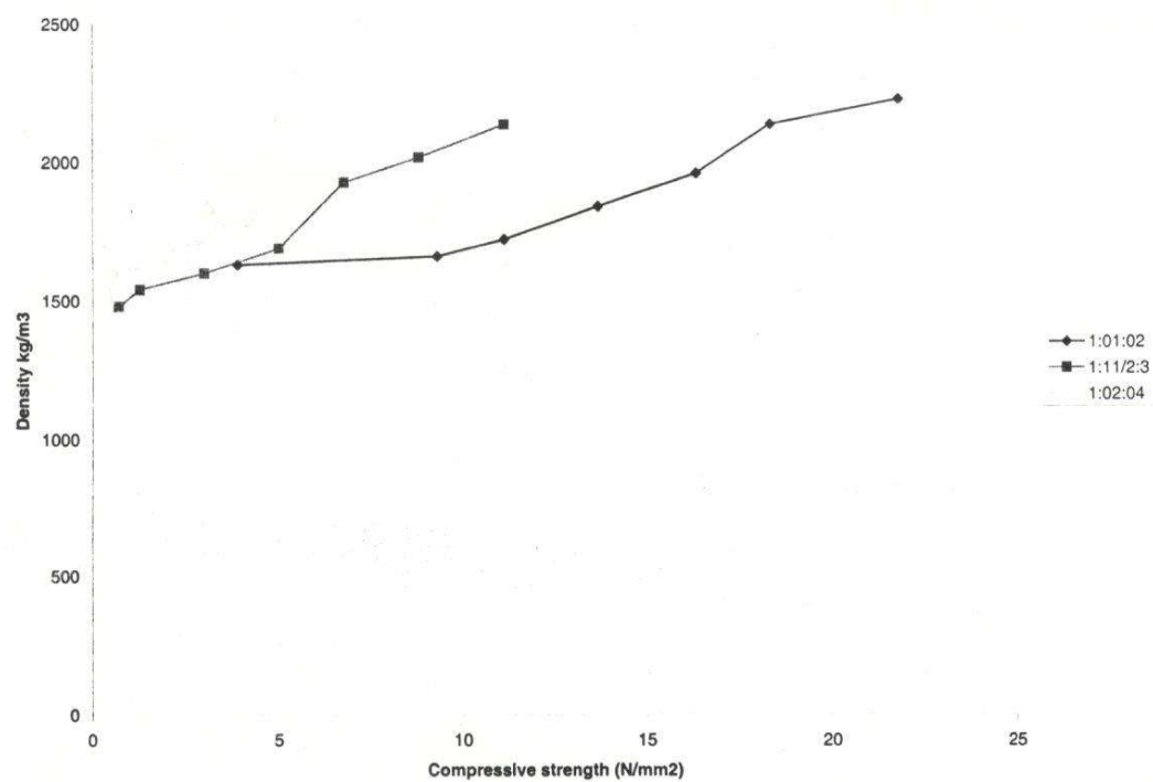
Figure 4: Density against compressive strength
