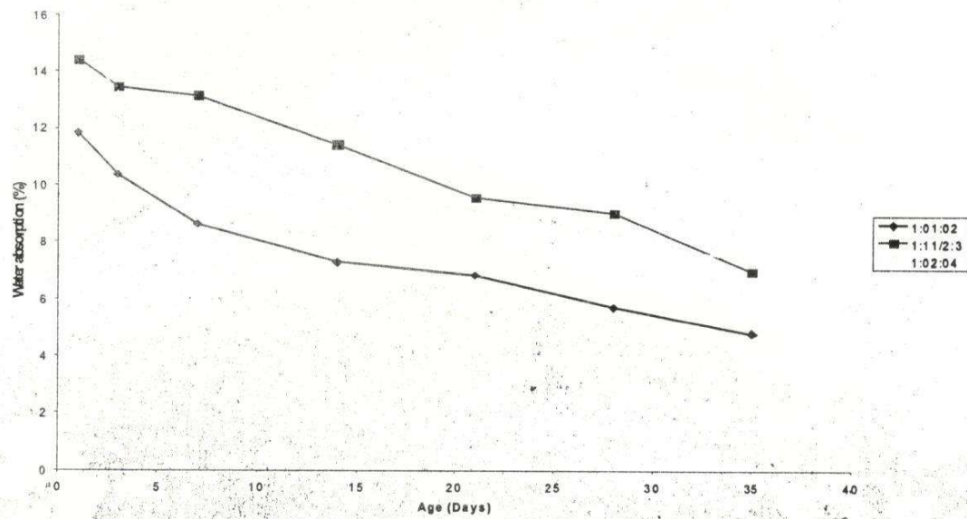
Figure 5: Water absorption against age
