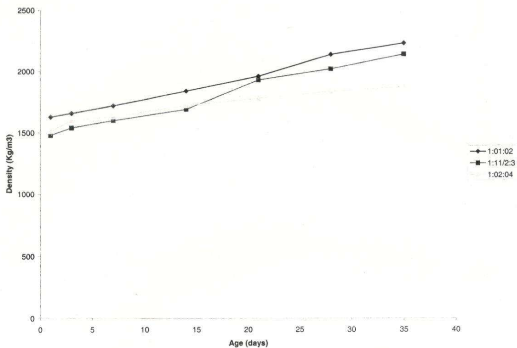
Figure 3: Density against age
