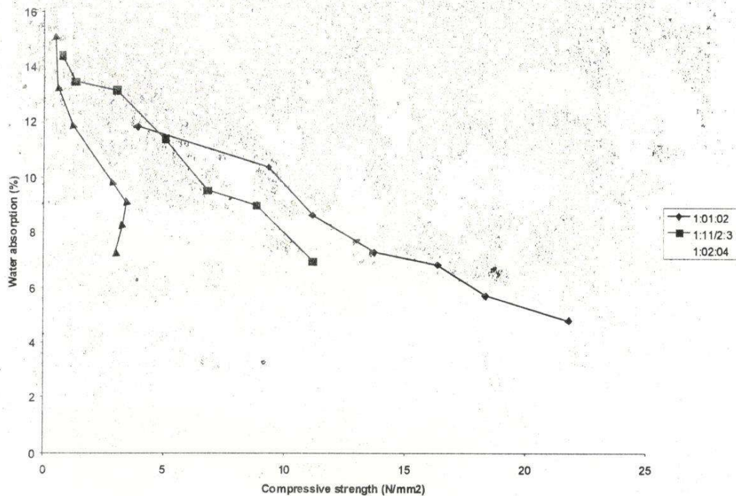
Figure 6: Water absorption against compressive strength
