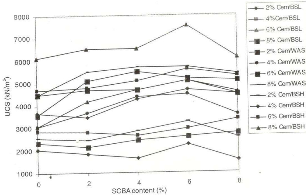
Fig. 6 Variation of UCS for 14 days Curing with SCBA at BSL, WAS and BSH Compaction Energy Level
