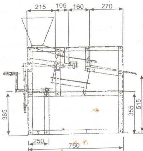
Figure 2: Orthographic view of the sieving machine
