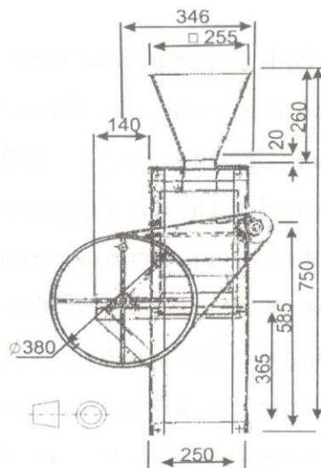
Figure 2: Orthographic view of the sieving machine
