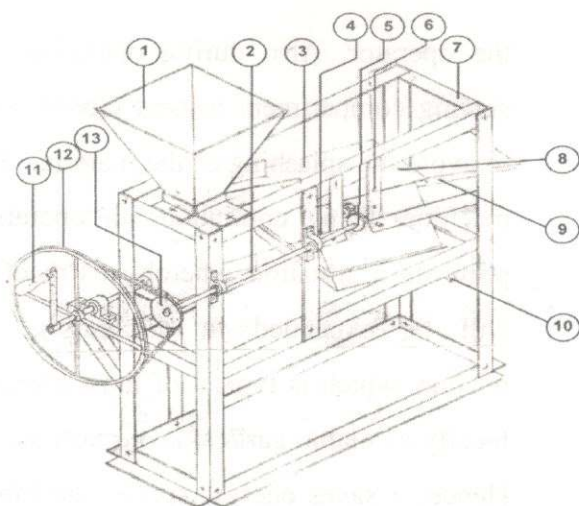
ure 1: Isometric view of the sieving machine
